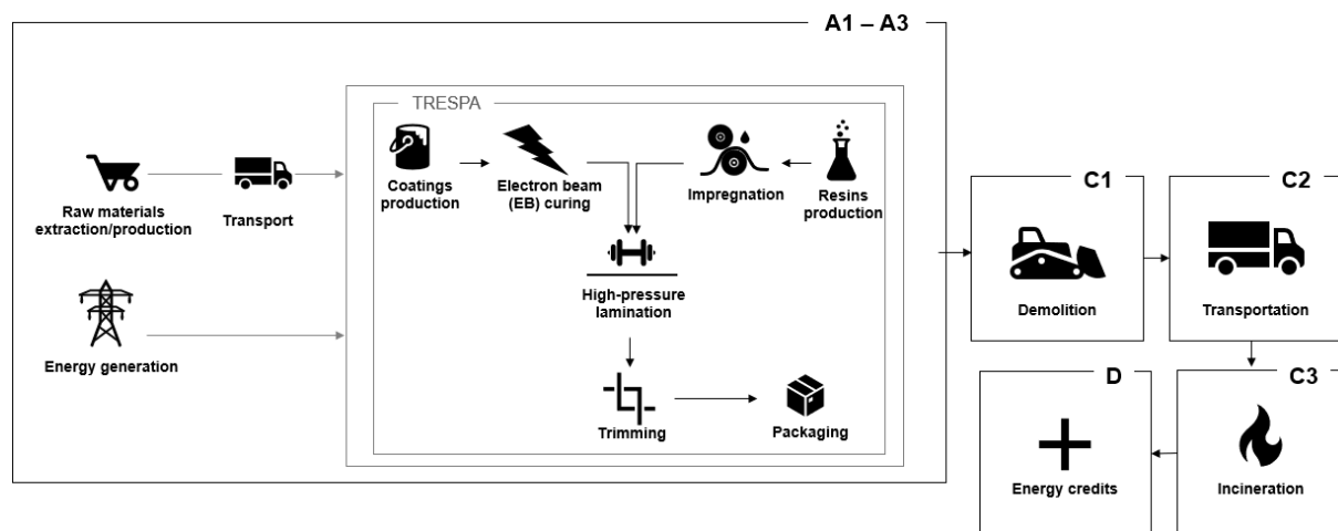
Figure 1: System boundary diagram for Trespa Meteon EDS grade 8mm
